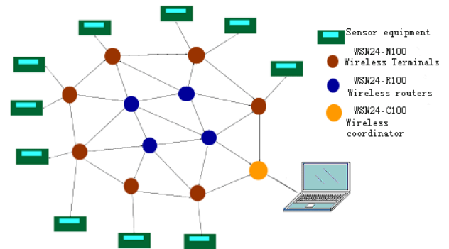
Figure1: Connection between nodes and end terminal by wireless network
